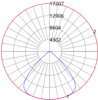
BAY-E-323/240W/8xx-U with optional field installed 90° lens
