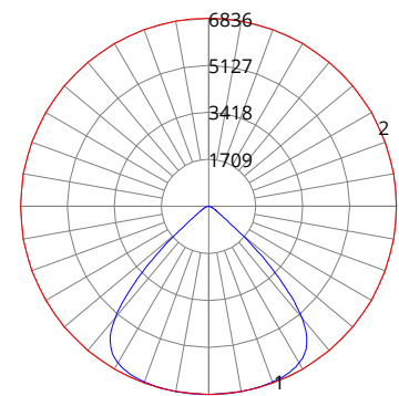
BAY-E-138/100W/8xx-U with optional field installed 90° lens
