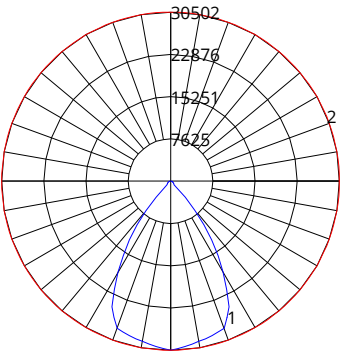
BAY-E-323/240W/8xx-U with optional field installed 60° lens
