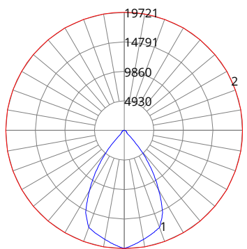
BAY-E-208/150W/8xx-U with optional field installed 60° lens
