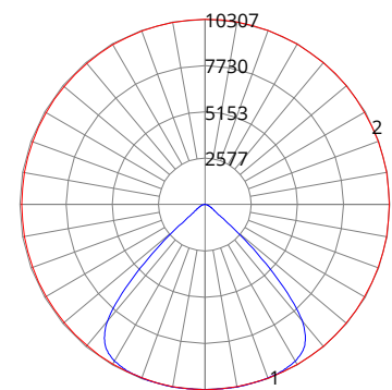
BAY-E-208/150W/8xx-U with optional field installed 90° lens
