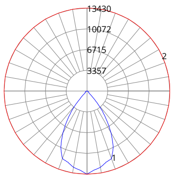
BAY-E-138/100W/8xx-U with optional field installed 60° lens
